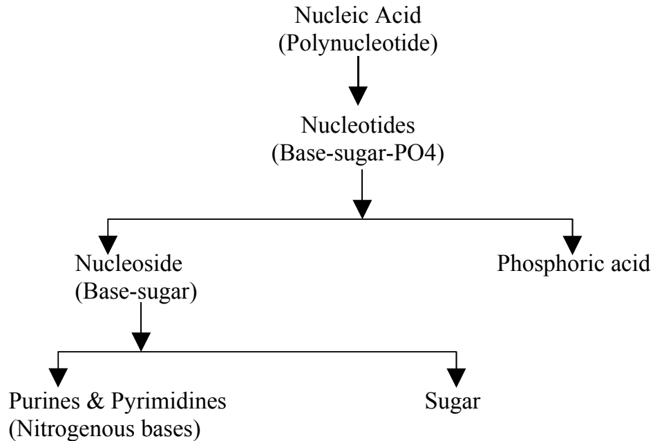
Figure 1 Components of Nucleic Acids
