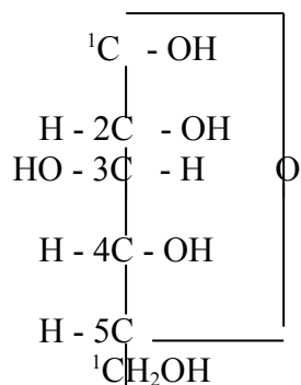
D – glucose (Fisher Projection)
