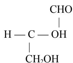
D-Glyceraldehyde
