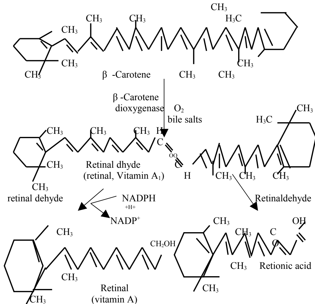
Figure 11 Formation of various forms of Vitamin A from the Vitamin A precursor- \beta -carotene
