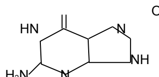
guanine
