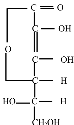
Figure 10: Chemical Structure of Vitamin C-Ascorbic Acid
