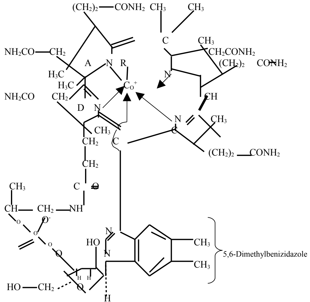
Figure 9 Chemical Structure of Cobalamin
