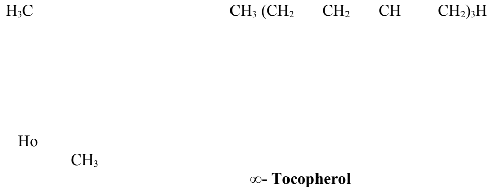
Figure 13 Chemical Structure of Vitamin E; \alpha -Tocopherol
