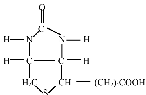
Figure 7 Chemical Structure of Biotin
