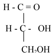
D-glycerose
