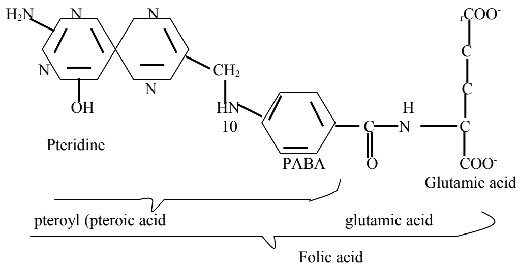
Figure 6 Chemical Structure of Folic Acid
