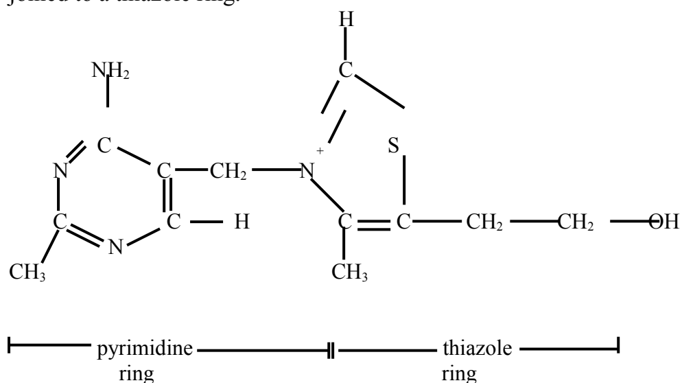
Figure 1: Vitamin B 1 - Thiamin
